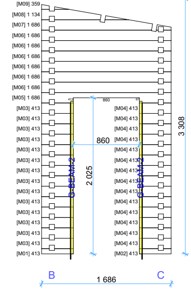
Wall N 1:50
