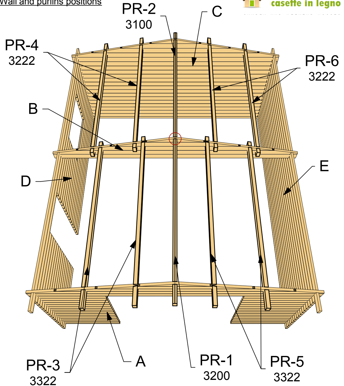
Wall and purlins positions
